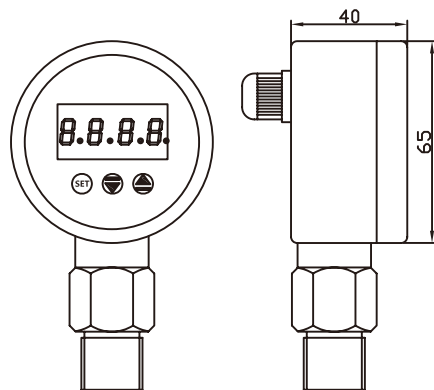
Radial installation
