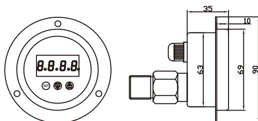
Axial installation
